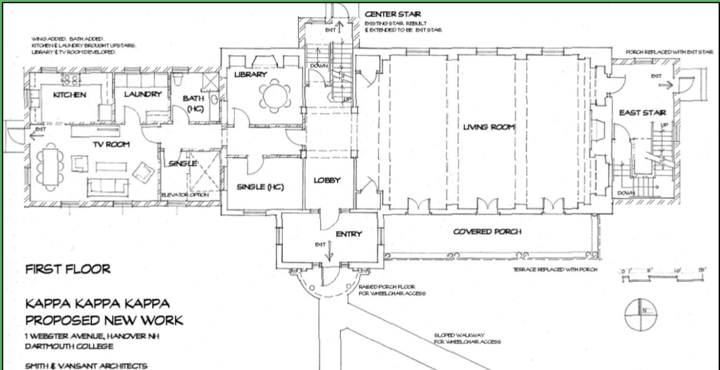
TRI-KAP BUILDING WITH PROPOSED ADDITIONS HANOVER, NH MAY 2006
